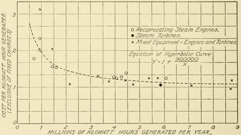
Fig. 165. Curve Showing the Total Cost per Kw. Hour Generated
